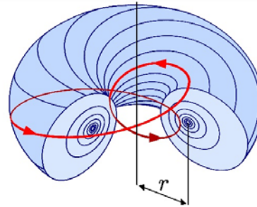
Figure 2: Schematic of the internal energy flow in the model. The lines of flow (geodesics) circulate twice around a family of nested toroidal surfaces before closing on themselves. The left-handed case is illustrated. For clarity, one complete double-loop path is emphasised. The toroidal structure is characterised by a length r = \lambda_c/4\pi .
