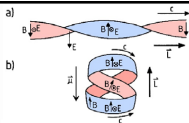
Figure 1: a) Twisted strip model for one wavelength of a photon with circular polarization in flat space. The \vec{B} -field is in the plane of the strip and the \vec{E} -field is perpendicular to it. b) A similar photon in a closed path in curved space with periodic boundary conditions of length \lambda_c . The \vec{E} -field vector is radial and directed inwards, and the \vec{B} -field is vertical. The magnetic moment \vec{\mu} , angular momentum \vec{L} , and direction of propagation with velocity c are also indicated.
